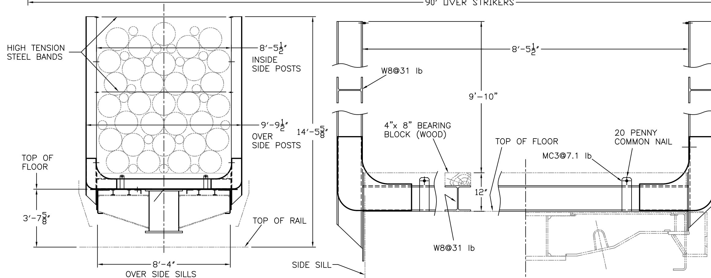
SECTION THROUGH LOADED CAR
